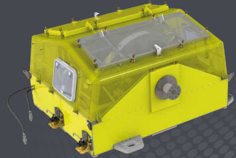
Power take off unit for Wave Energy Converter
