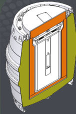
Impact simulation for radioactive container
