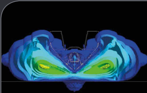
Model of pressure wave intensity during blast test
